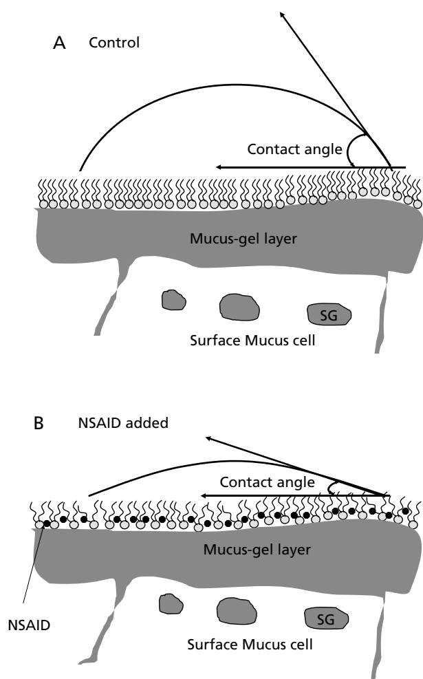
Figure 1 Schematic molecular model of putative PC-enriched monolayer at the interface between the gastric mucus gel and the gastric juice to provide an acid repellent surface hydrophobic barrier. This property can be determined by measuring the contact angle at the air-liquid-solid interface. Schematic depiction of the hydrophobic properties of the gastric mucosa under control conditions (A) (contact angle readings between 60–80°) and after the stomach has been exposed to a luminal NSAID and surface hydrophobicity is reduced (B) (contact angle readings <40°).
